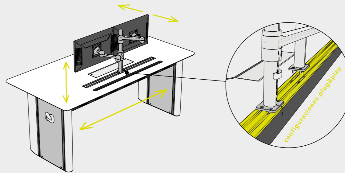
Regulation system using aluminium rail on work surface.
